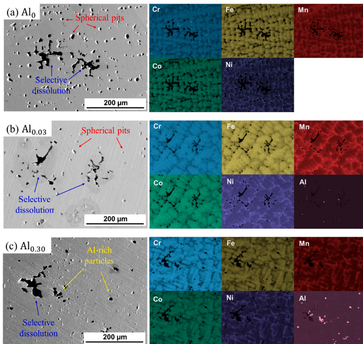
Fig. 8. SEM micrographs and EDX mapping of the corroded surfaces of CrMnFeCoNiAl x ( x = 0, 0.03, 0.30 ) high-entropy alloys (a) Al 0 , (b) Al 0.03 and (c) Al 0.30 after cyclic polarisation testing.
