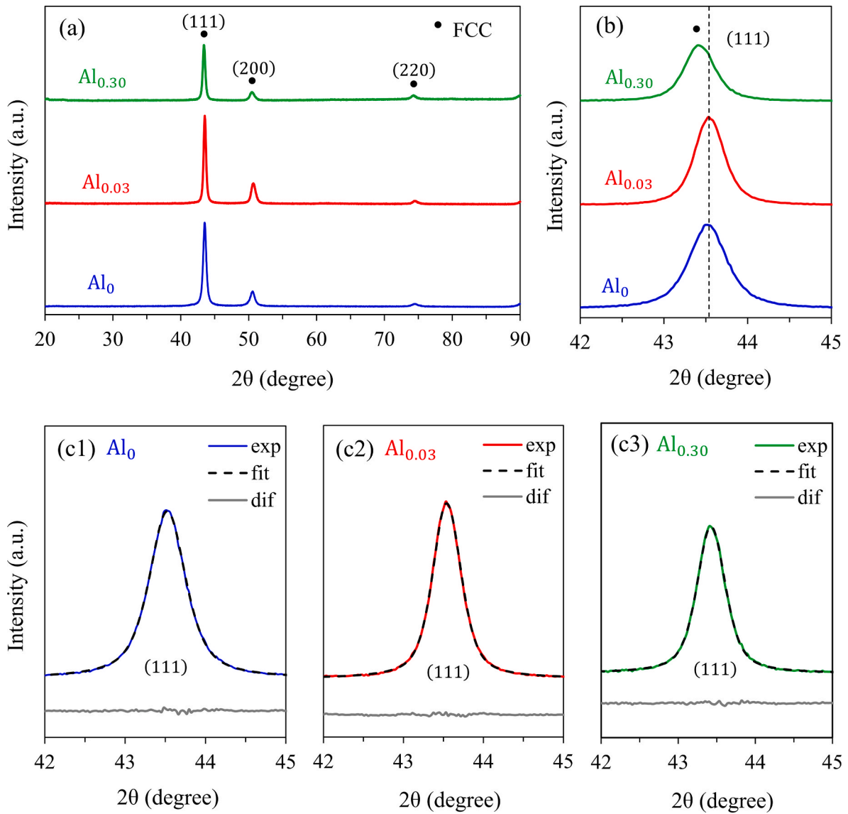
Fig. 2. (a) XRD patterns of as-cast \text{CrMnFeCoNiAl}_x ( x = 0, 0.03 , and 0.30 ) high-entropy alloys. (b) Magnified pattern showing peak shifting with Al addition. Bragg peaks of the FCC (111) plane reflection fitted with a Pseudo-Voigt function for (c1) \text{Al}_0 , (c2) \text{Al}_{0.03} and (c3) \text{Al}_{0.30} .
