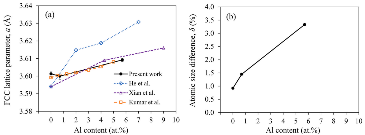
Fig. 3. (a) Evolution of the FCC lattice constant and (b) the atomic size difference parameter ( \delta ) with Al content (at.%) in the \text{CrMnFeCoNiAl}_x ( x = 0, 0.03, 0.30 ) high-entropy alloys. Data from Refs. [25,26,35] are included for comparison.
