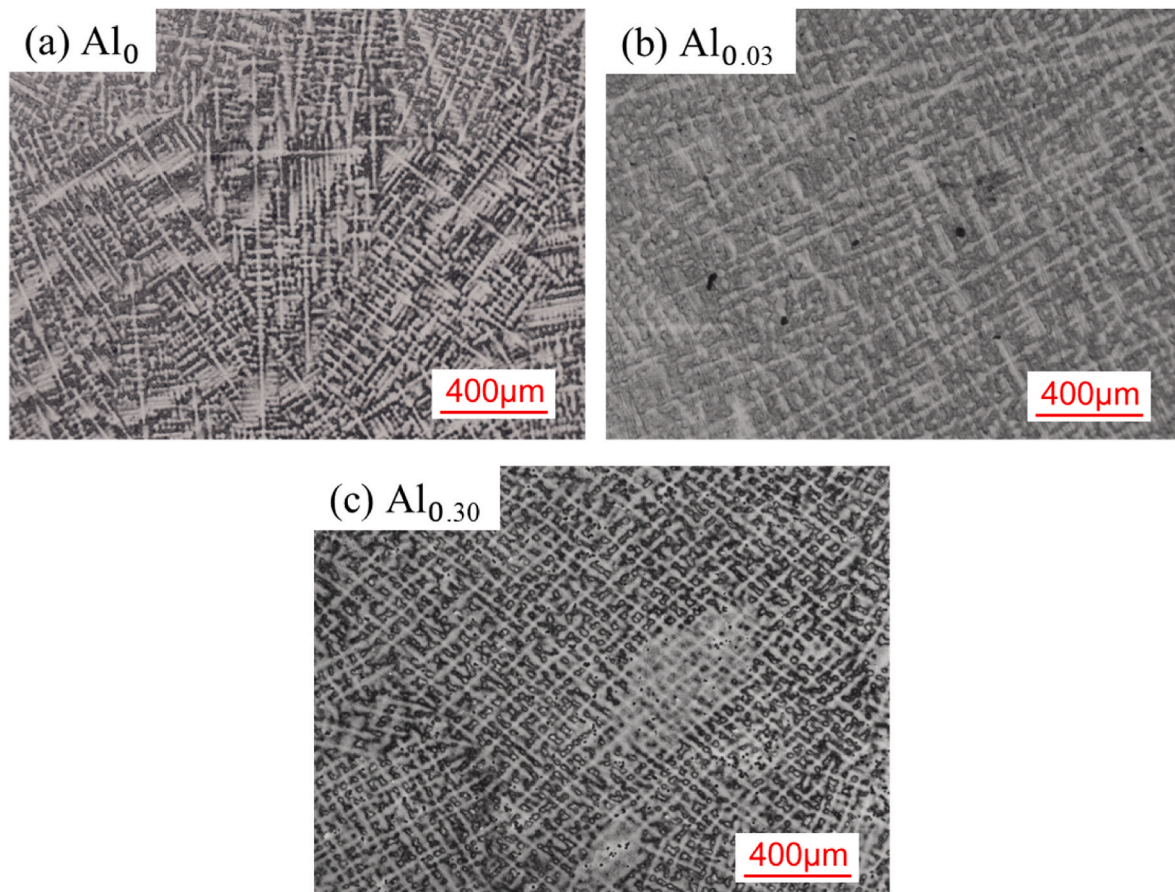
Fig. 4. Optical microscope micrographs of as-cast CrMnFeCoNiAl x (x = 0, 0.03, 0.30) high-entropy alloys (a) Al 0 , (b) Al 0.03 and (c) Al 0.30 .
