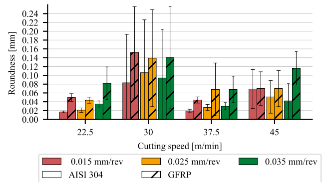
Fig. 10. Roundness [mm].
