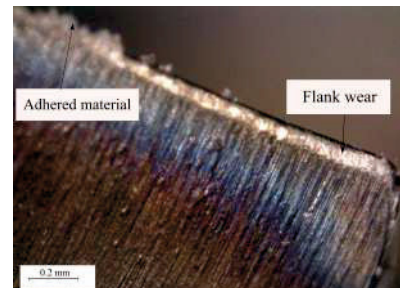
Fig. 5. Cutting lips view after 9 holes.
