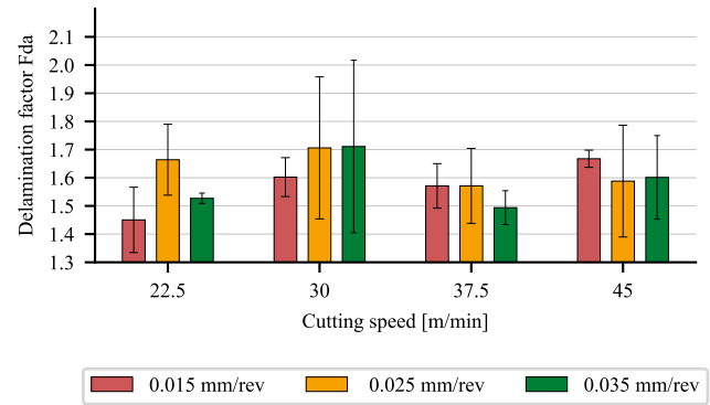
Fig. 7. Delamination factor F_{da} measurements.
